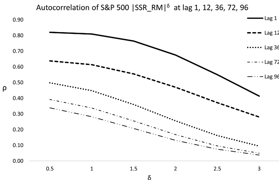
FIGURE 4 Autocorrelation of S&P 500 |SSR\_RM_i|^{\delta_R} at lags 1, 12, 36, 72, 96
